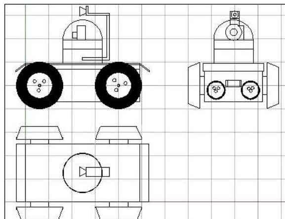
Figure 7. CAD design of the robot
