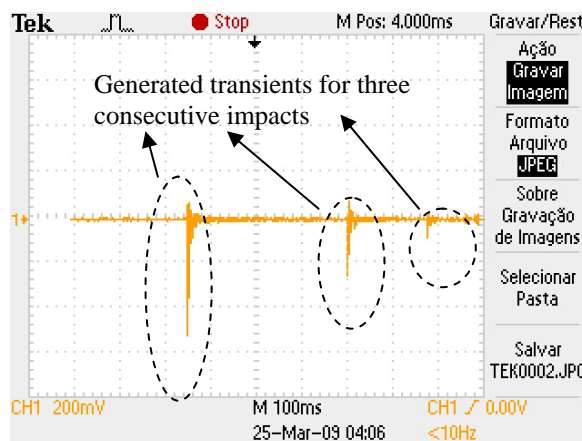
Figure 2: Signal generated by 3 consecutive impacts of a resin ball.
