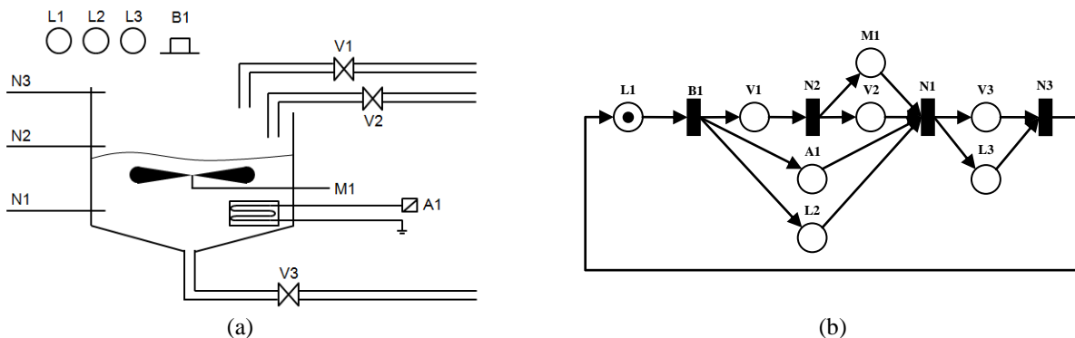
Figure 5.1. (a) Example of mixing system (based on Miyagi (1996)), (b) Petri net describing the control logic of the mixer system.
