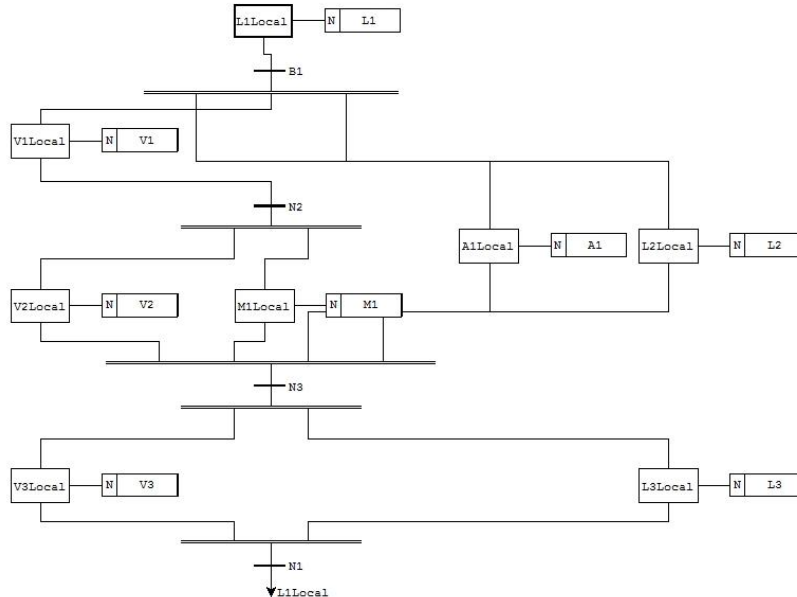
Figure 5.3. SFC diagram generated by transcription tool and displayed in Beremiz.
