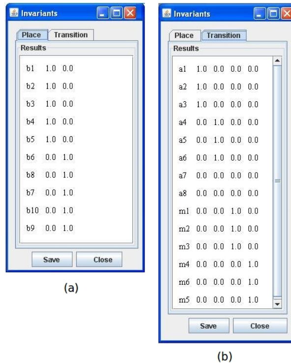
Figure 5. (a) Place invariants and (b) transition invariants obtained by the GHENeSys system.
