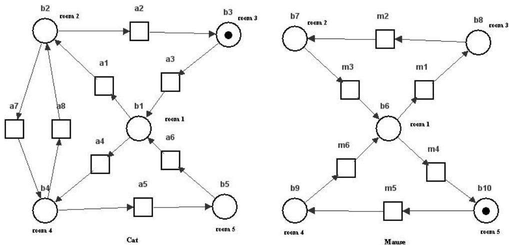
Figure 3. Modelling in GHENeSys the cat and mouse problem.
