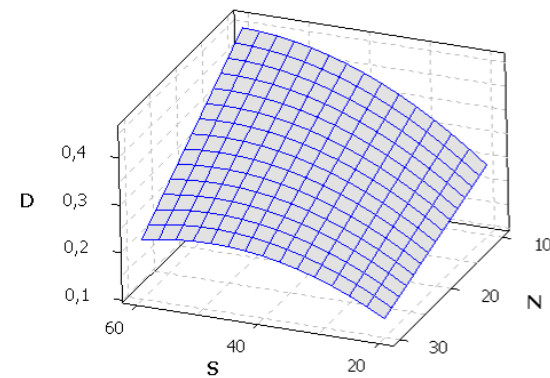
Figure 11 – Interaction effect between welding speed and contact tip to workpiece distance on dilution (W f = 8.5 m/min; V = 29.5 V)
