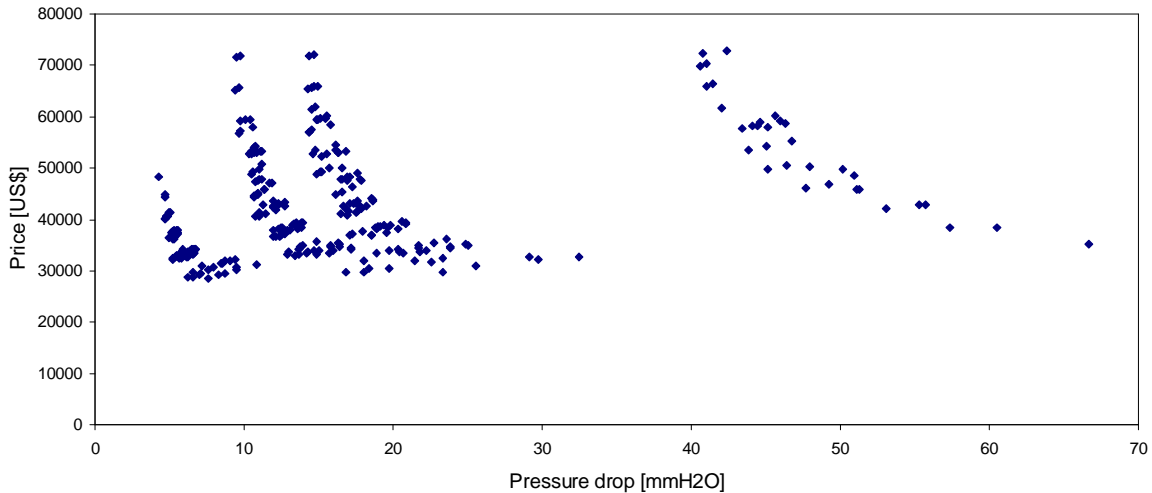
Figure 7. Graphic price versus pressure drop in the evaporator
