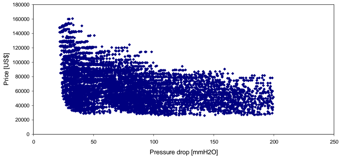
Figure 5. Graphic of price versus pressure drop in the condenser
