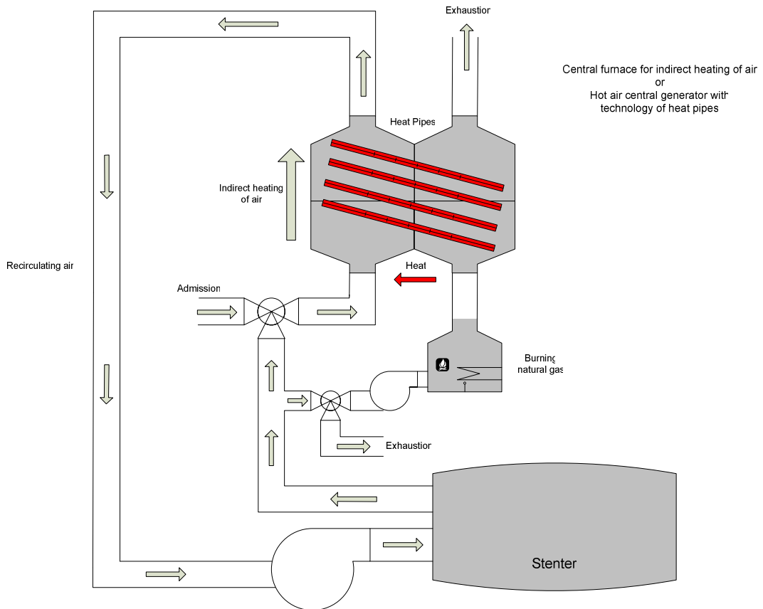
Figure 1. Proposed indirect heating system for stenters with pre-heating of combustion oxidizer
