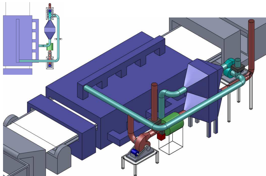
Figure 2. Layout of the proposed air heating system for stenters
