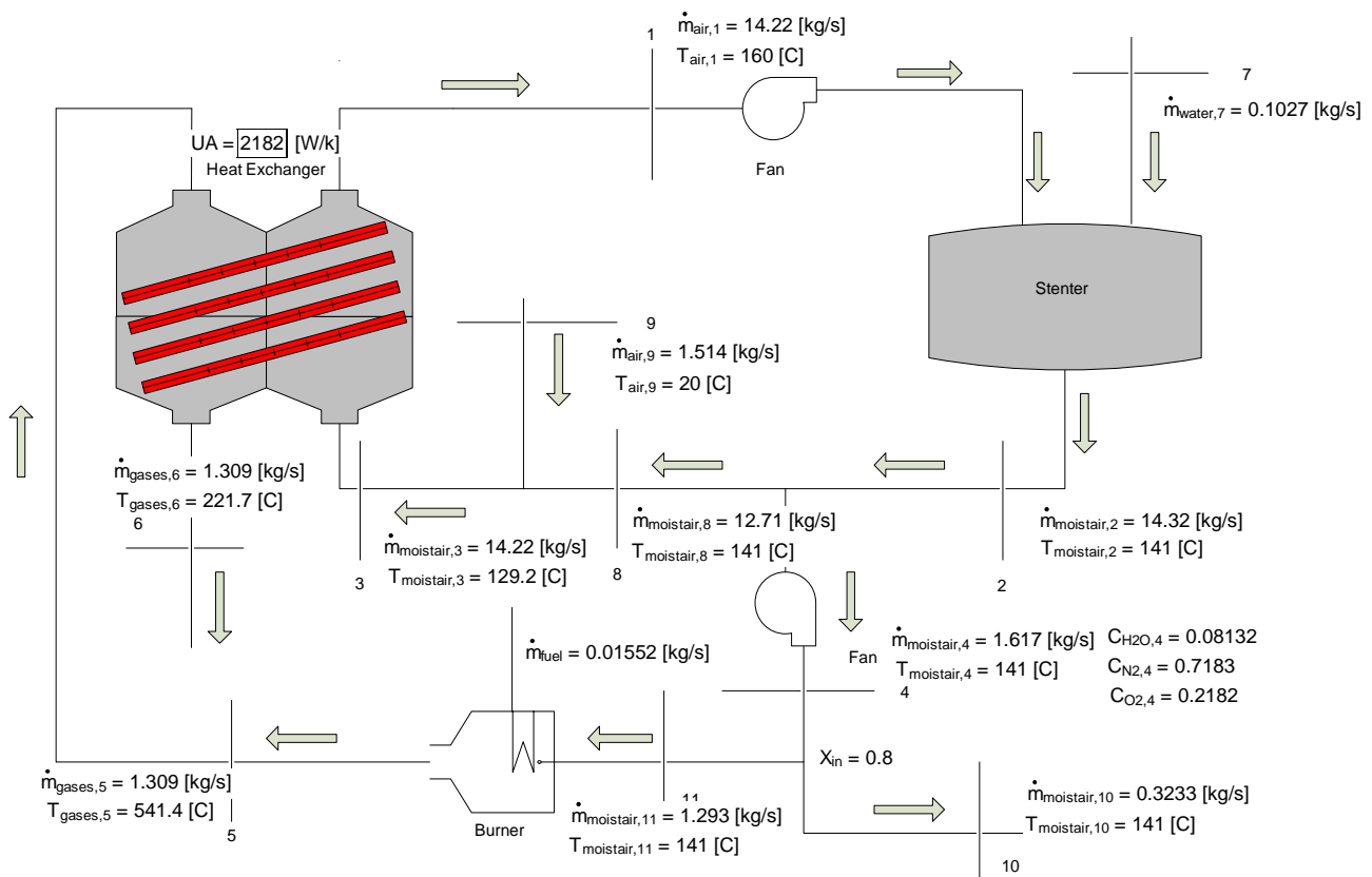
Figure 4. Interface input and output of the ESS program to calculate the balance of mass and energy
