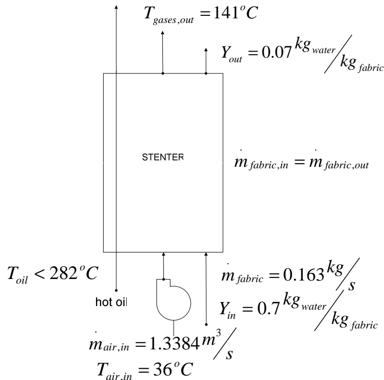
Figure 3. Stenter chosen for case study
