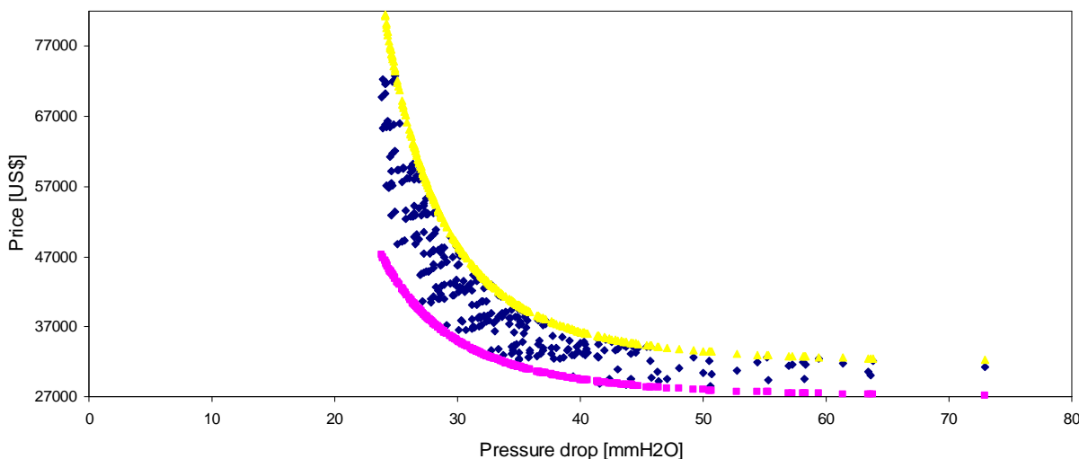
Figure 6. Points near the lower envelope
