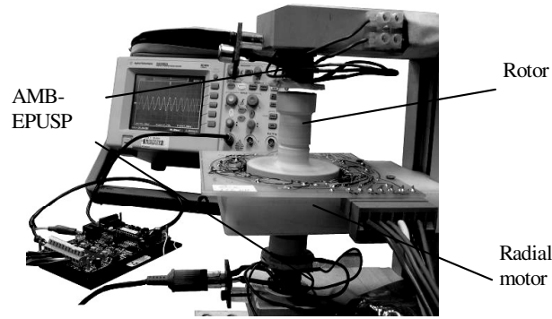
(a) Set-up
