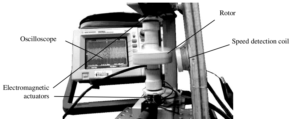
Figure 5. Set-up for testing the magnetic suspension.
