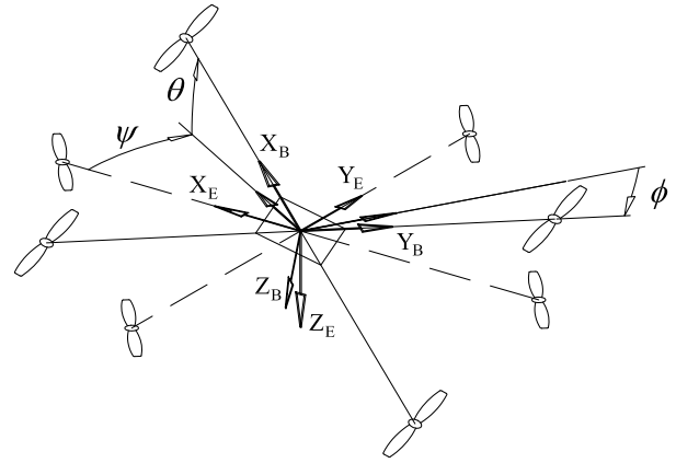
Figure 2. Euler Angles - Rotation
