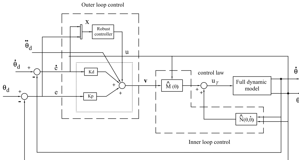
Figure 3. Inverse Dynamic Control, Imperfect Compensation
