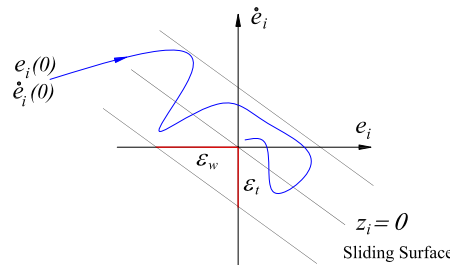
Figure 4. Error Trajectory with Robust Control and Chattering Elimination
