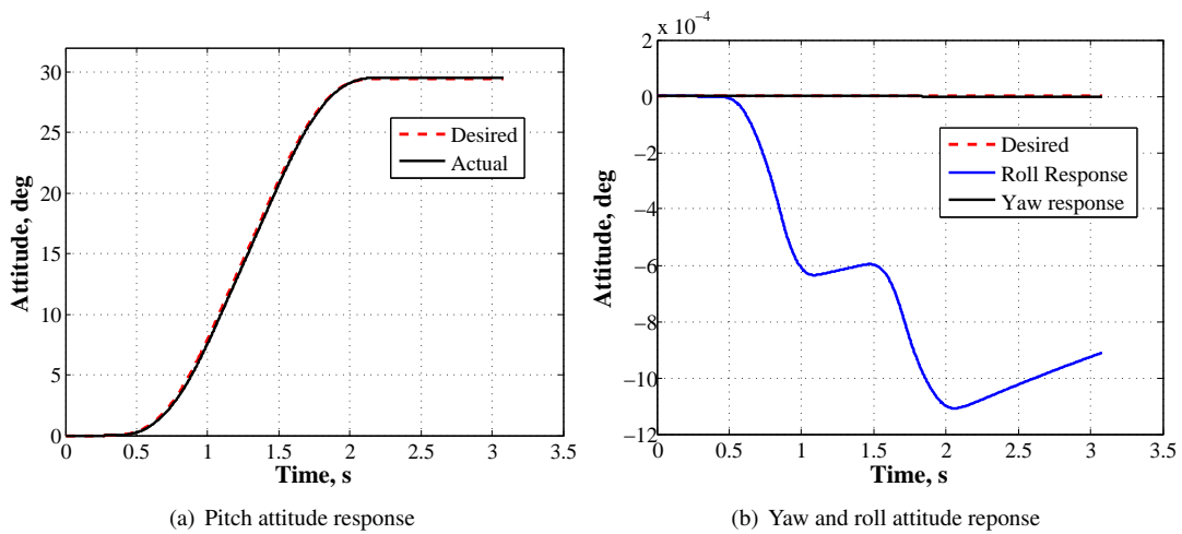
Figure 5. Quadrotor response
