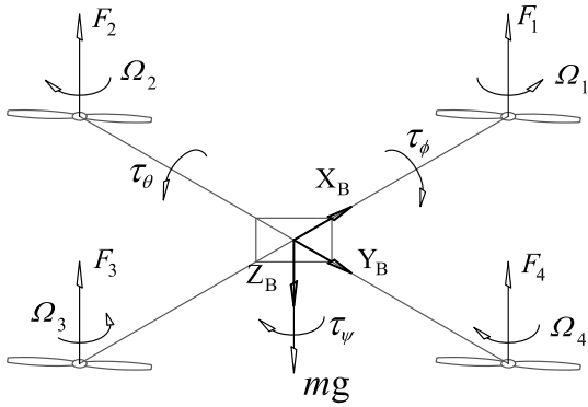
Figure 1. Quadrotor Configuration
