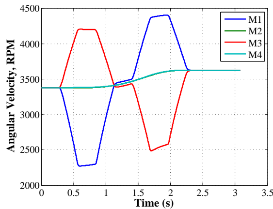
Figure 6. Propeller angular velocities
