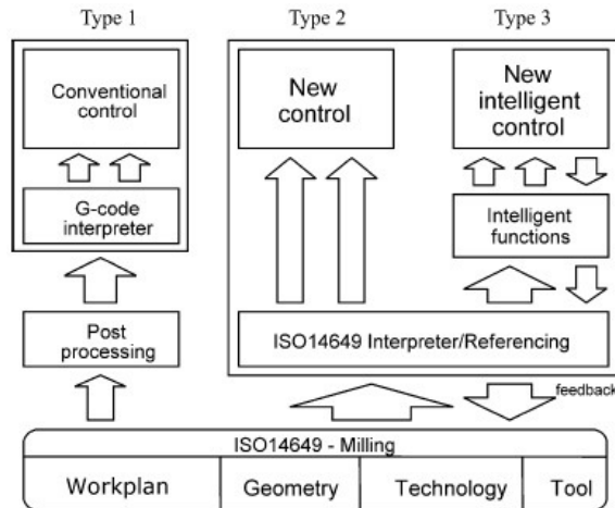
Figure 4. Types of STEP-NC controllers (Suh et al. , 2003)
