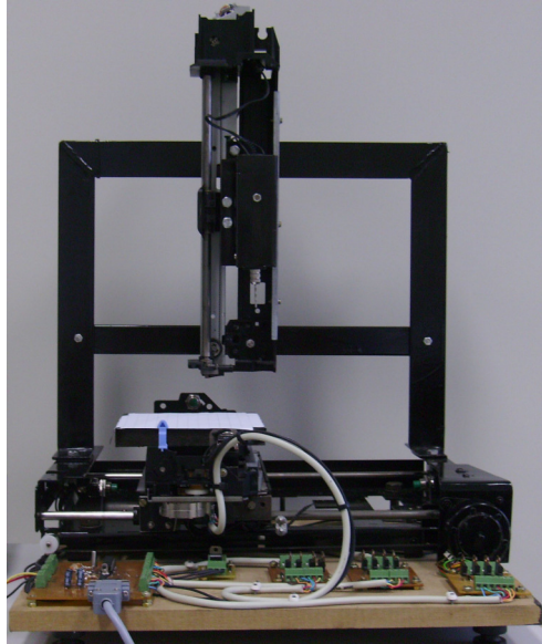
Figure 6. CNC drilling device adherent to STEP-NC
