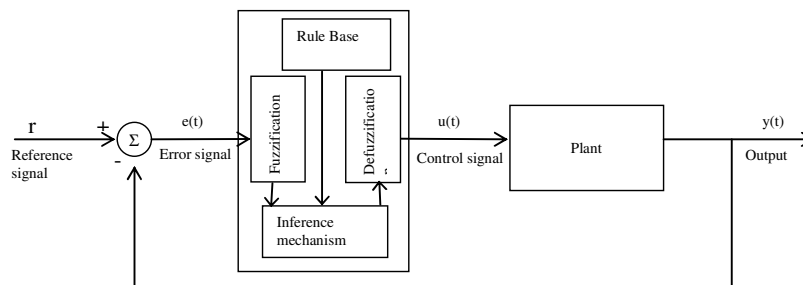
Figure 2. Fuzzy controller inserted in the control loop
