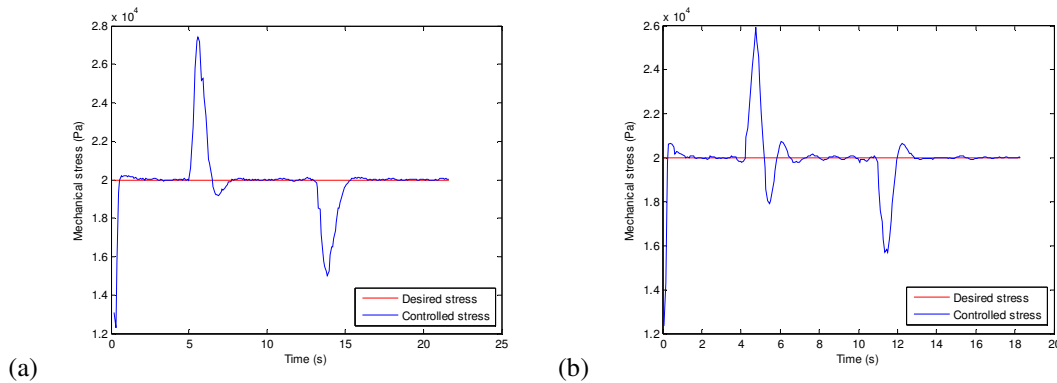
Figure 6. Disturbances at: (a) Fuzzy controller PD + I and (b) PID Controller.
