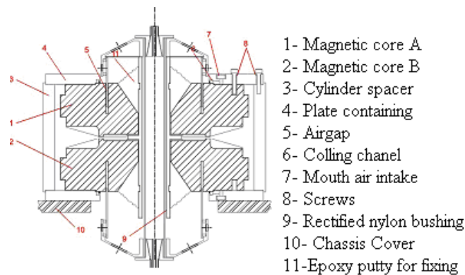
Figure 1. Parts of a generic electrodynamic shaker.
