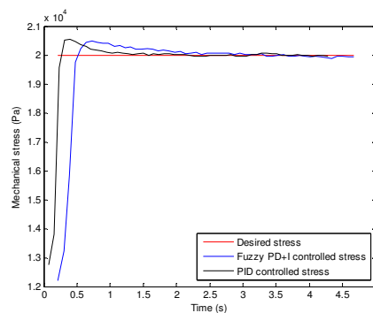
Figure 8. Comparison between PID and fuzzy controllers.
