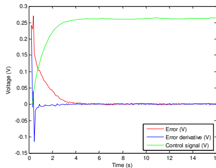
Figure 7. Control signal, error and derivative of error.
