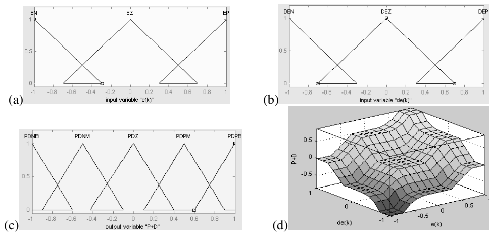
Figure 3. Membership functions for two inputs (a) e(t) and (b) de(t) , control output (c) u_F(t) and (d) fuzzy control surface of the Fuzzy PD-controller.
