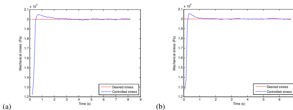
Figure 5. (a) Fuzzy controller PD + I and (b) PID controller.
