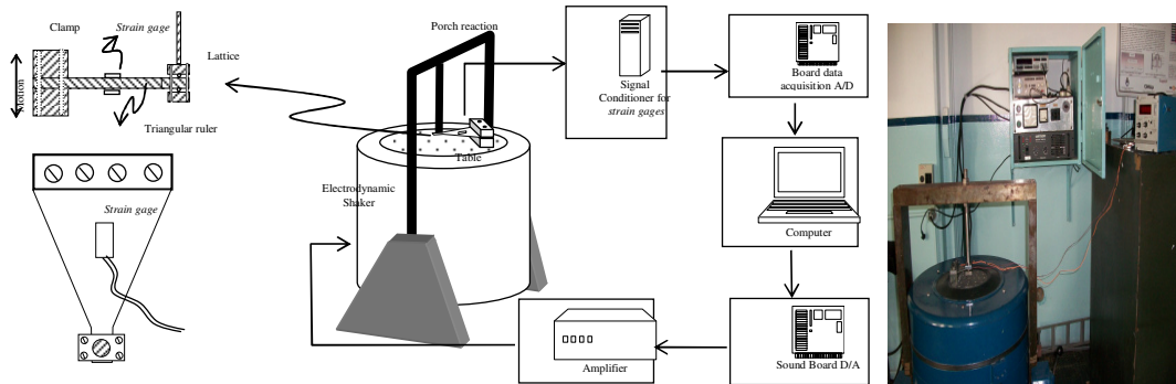
Figure 4. Scheme of control system and photo of the prototype tested.
