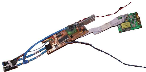
Figure 7. Pitot's internal transmitter system (without the battery)
