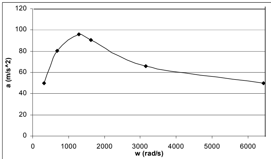
Figure 3 - Typical Acceleration x Frequency curves for the shaker.
