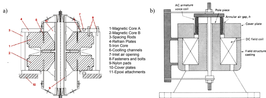
Figure 1. Sketch and setups of typical electrodynamic shakers
