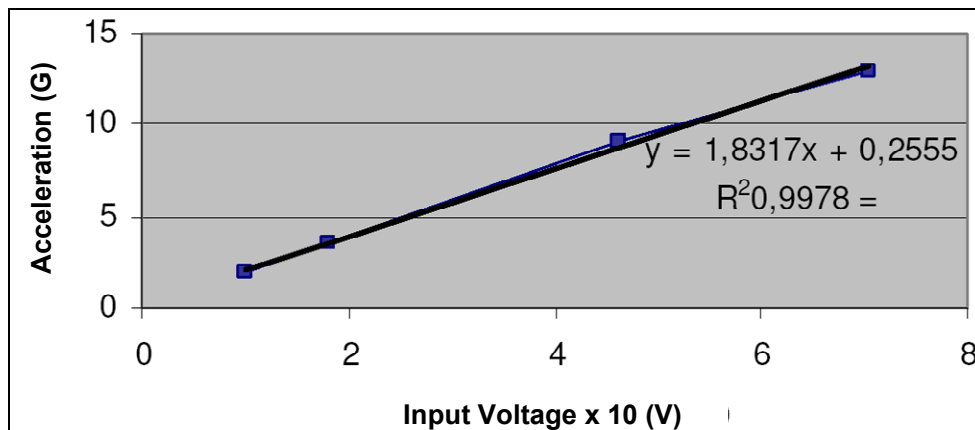
Figure 4 - Typical plot for amplifier voltage output versus measured acceleration on shaker's table (without test specimen)
