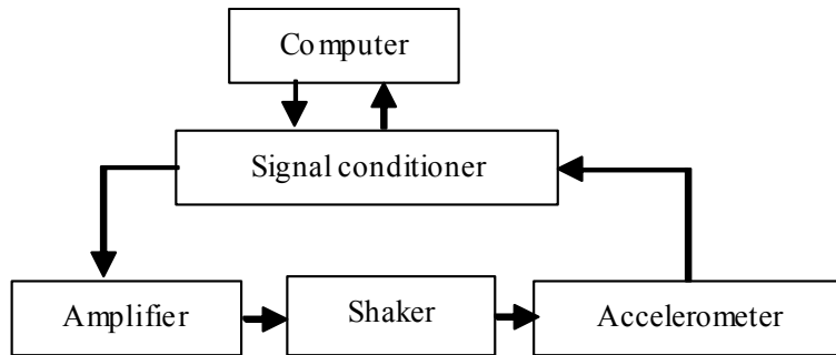
Figure 3. Closed Loop Scheme for the Active Control
