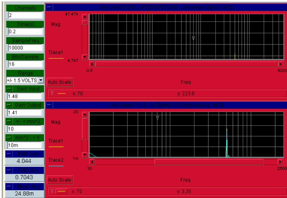
Figure 7. Acceleration PSD for single sine at 500Hz and acceleration amplitude of 1 m/s 2 ( 0.707 m/s 2 RMS)
