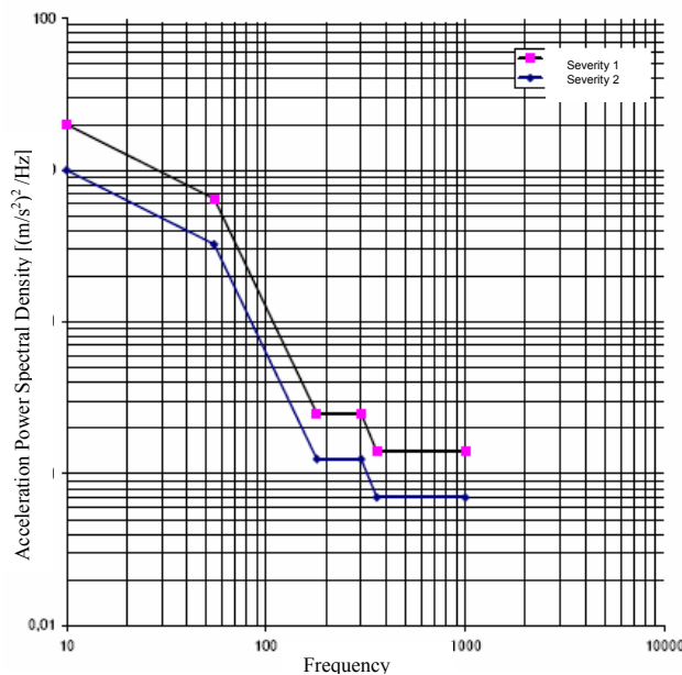
Figure 2. Plot for Acceleration Power Spectral Density versus frequency (Volkswagen Standard, 2004)
