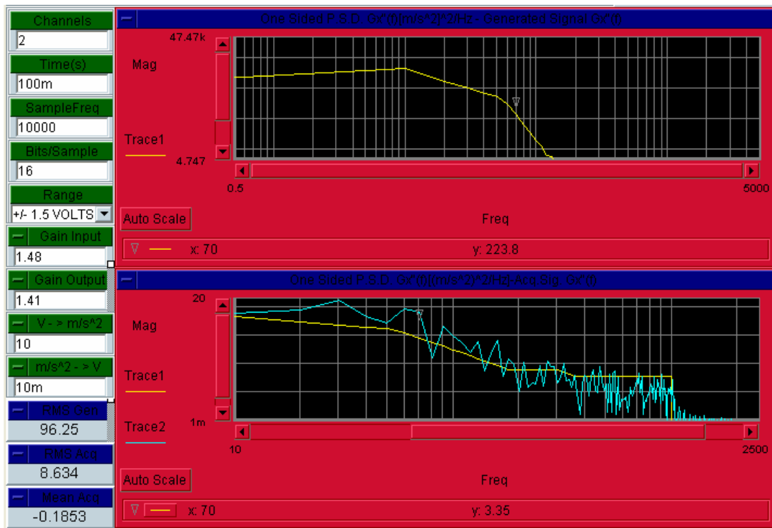
Figure 8 - Acceleration PSD for random vibration test with severity level 3 (13.9 m/s 2 RMS acceleration) (Volkswagen Standard (2004))
