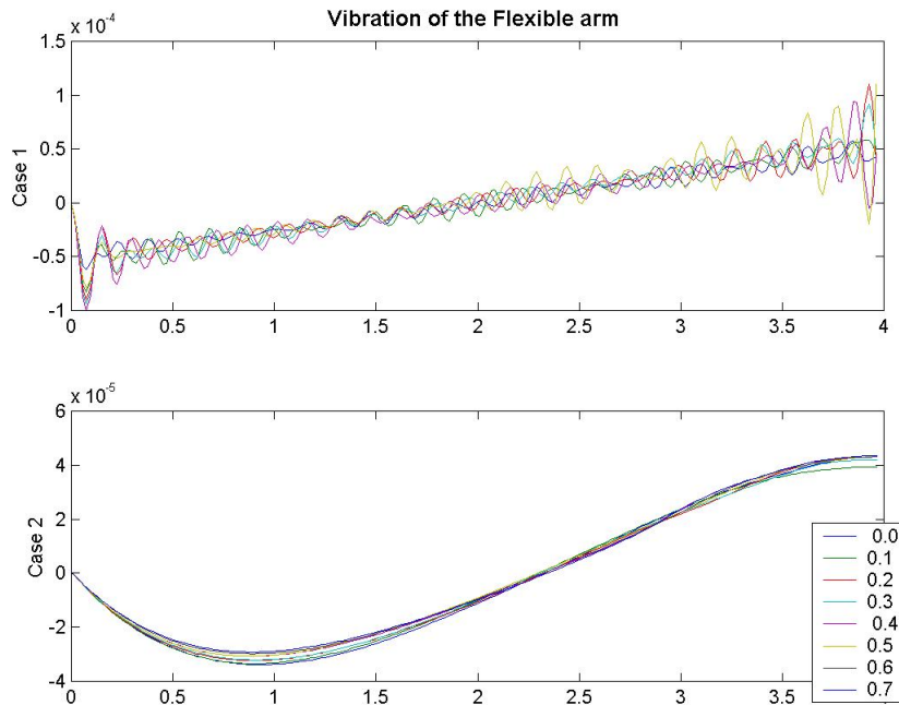
Figure 3. Arm Tip Vibration
