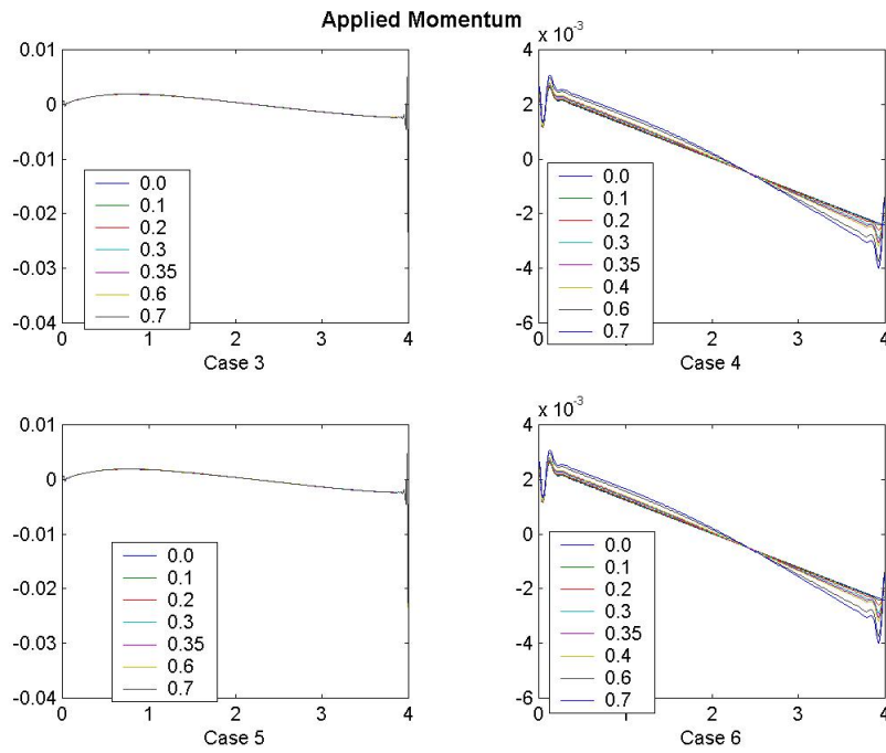
Figure 9. Torque applied to the hub
