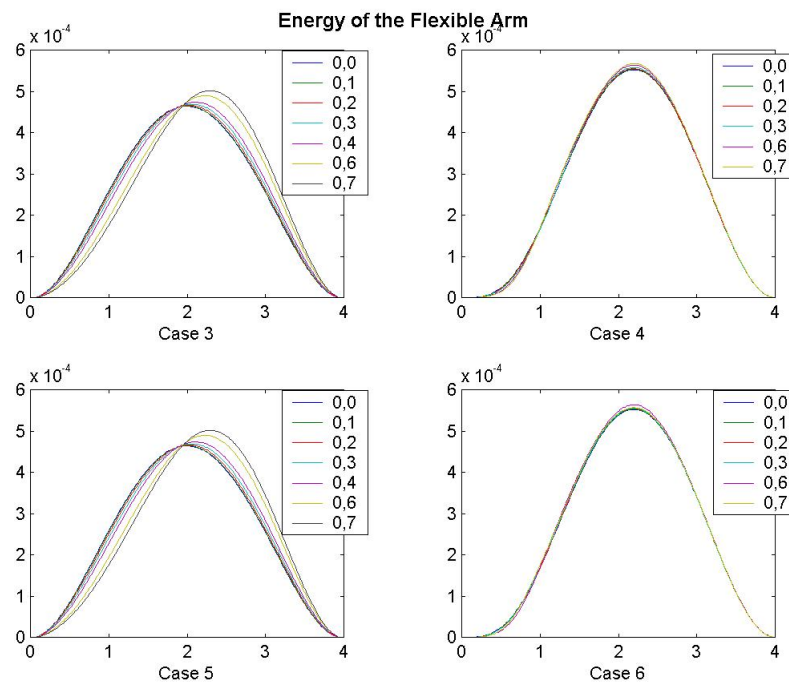
Figure 11. Total energy demanded for the flexible mechanism
