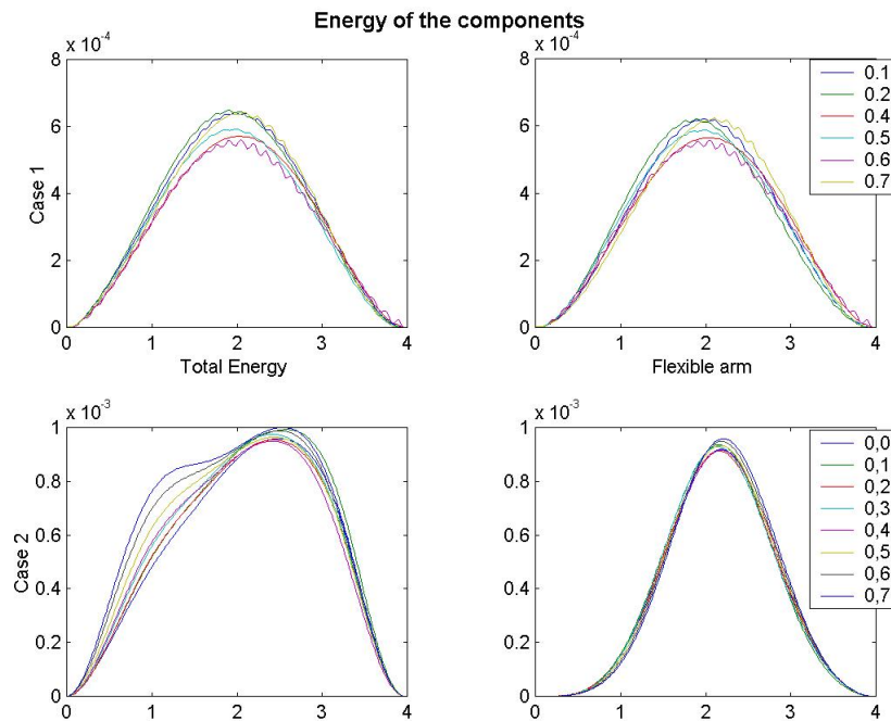
Figure 6. Energy delivered to slider movements
