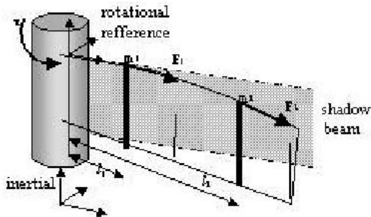
Figure 2. Deformed and Shadow Beam corresponding to the flexible arm
