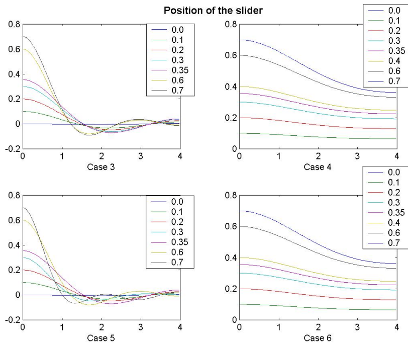
Figure 8. Position of the sliders during the manoeuvre
