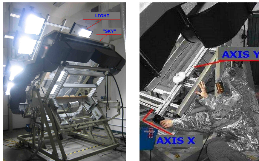
Figure 1. (a) Solar Simulator (b) Manual cartesian positioner /pyranometer/tecnician.
