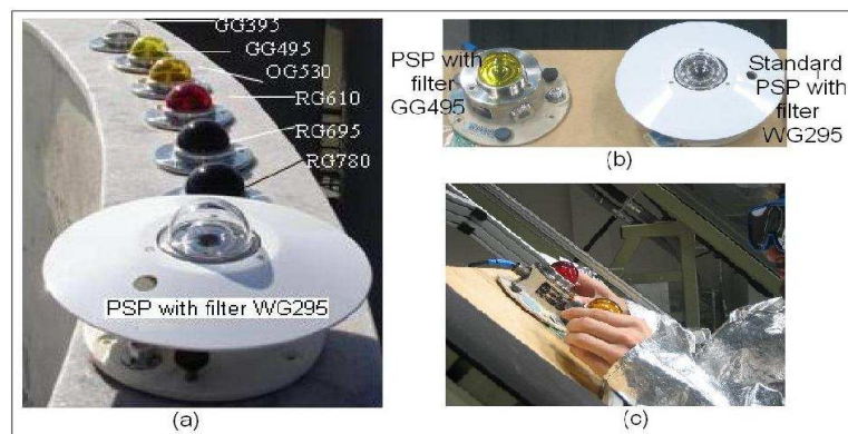
Figure 6. (a) Filters used; (b) Sensor on benchmark of solar simulator; (c) Substitution of filters during test.
