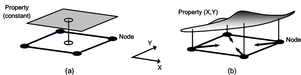
Figure 2. Properties at the element level. (a) Homogeneous Finite Element (HFE); (b) Graded Finite Element (GFE)
