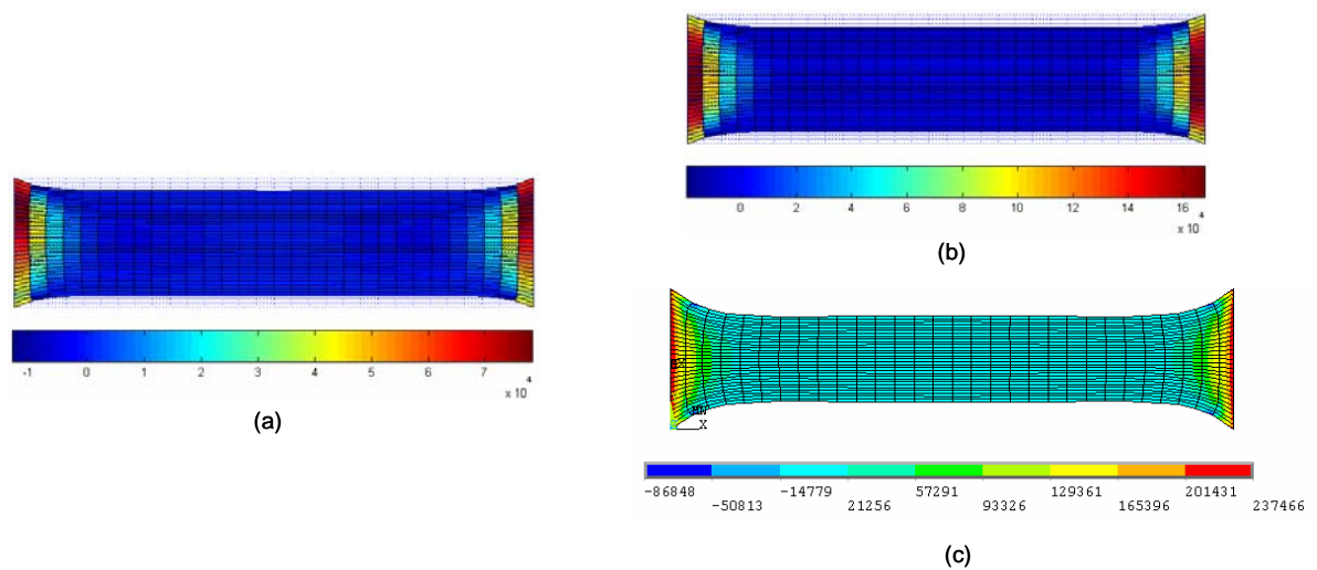
Figure 6. Stress \sigma_{zz} ( Pa ). (a) FGP model with Matlab; (b) Non-FGP model with Matlab; (c) Non-FGP model with Ansys
