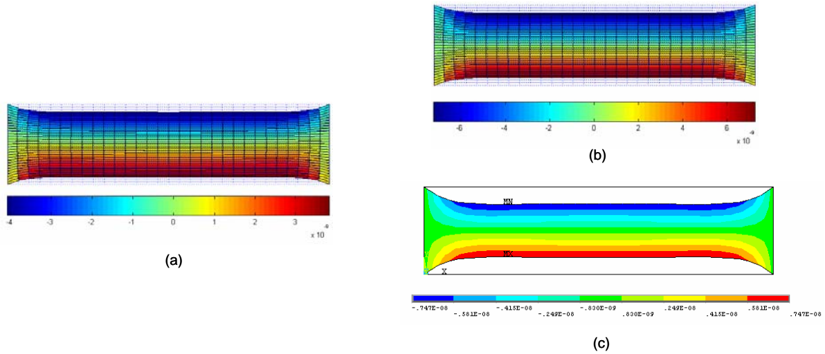
Figure 4. Vertical Displacement ( m ). (a) FGP model with Matlab; (b) Non-FGP model with Matlab; (c) Non-FGP model with Ansys
