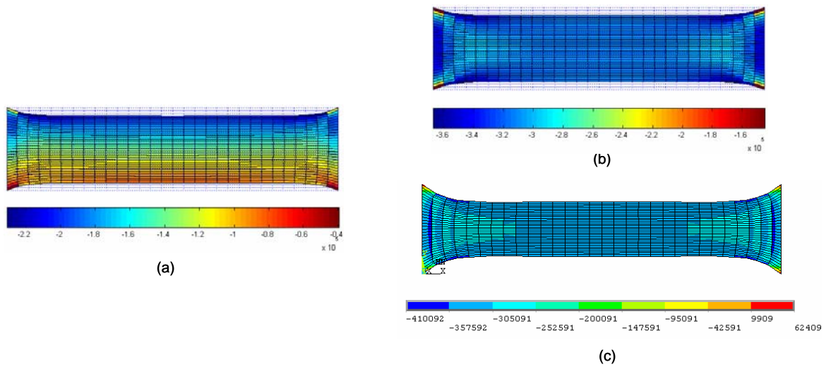
Figure 5. Stress \sigma_{xx} ( Pa ). (a) FGP model with Matlab; (b) Non-FGP model with Matlab; (c) Non-FGP model with Ansys
