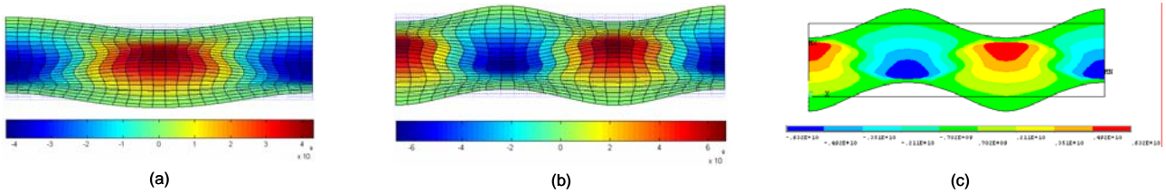
Figure 10. Second piezoelectric mode. (a) FGP model with Matlab; (b) Non-FGP model with Matlab; (c) Non-FGP model with Ansys
