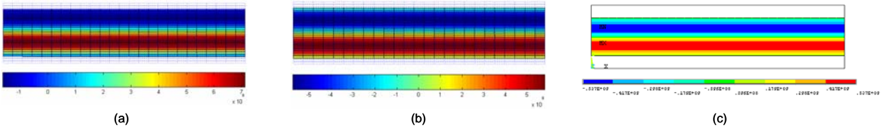
Figure 9. First piezoelectric mode. (a) FGP model with Matlab; (b) Non-FGP model with Matlab; (c) Non-FGP model with Ansys
