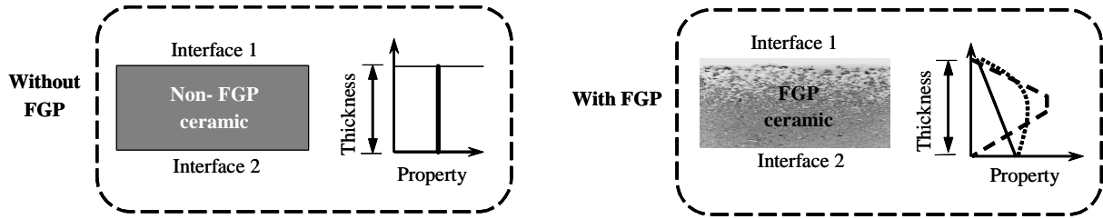
Figure 1. Sketch of a traditional (non-FGP) piezoelectric ceramic and of a FGP piezoceramic disk
