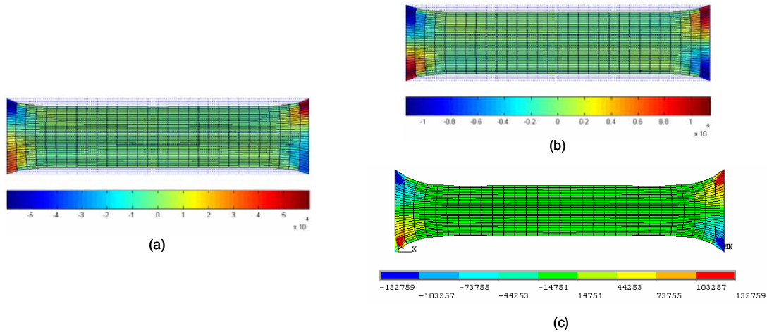
Figure 7. Stress \sigma_{xz} (Pa). (a) FGP model with Matlab; (b) Non-FGP model with Matlab; (c) Non-FGP model with Ansys
