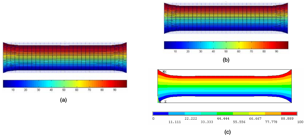
Figure 8. Electric potential (V). (a) FGP model with Matlab; (b) Non-FGP model with Matlab; (c) Non-FGP model with Ansys
