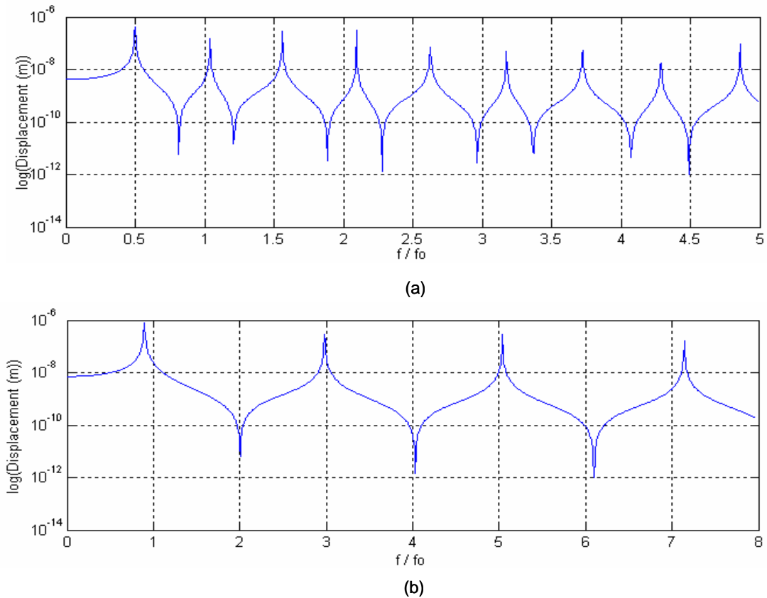
Figure 11. Displacement frequency response. (a) FGP model with Matlab; (b) Non-FGP model with Matlab
