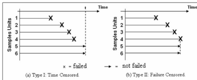
Figure 5. Censored Data (Krishnamoorthi, 1992)
