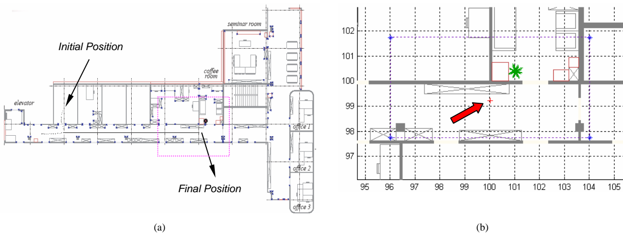
Figure 4. The robot assumed trajectory in the ASL environment map (a) and detail of the final position of the robot according to the planned trajectory path (b) – red cross.
