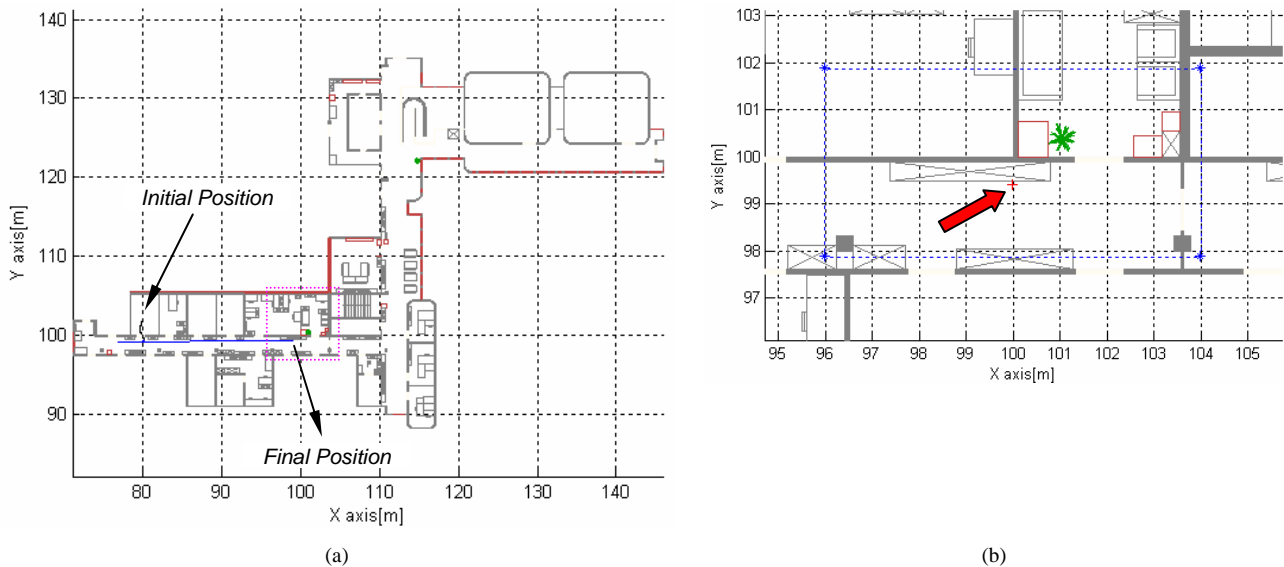
Figure 7. Trajectory estimation obtained from fusion of system state predictions by laser scan data and omni-directional camera images (a) and final robot position found.
