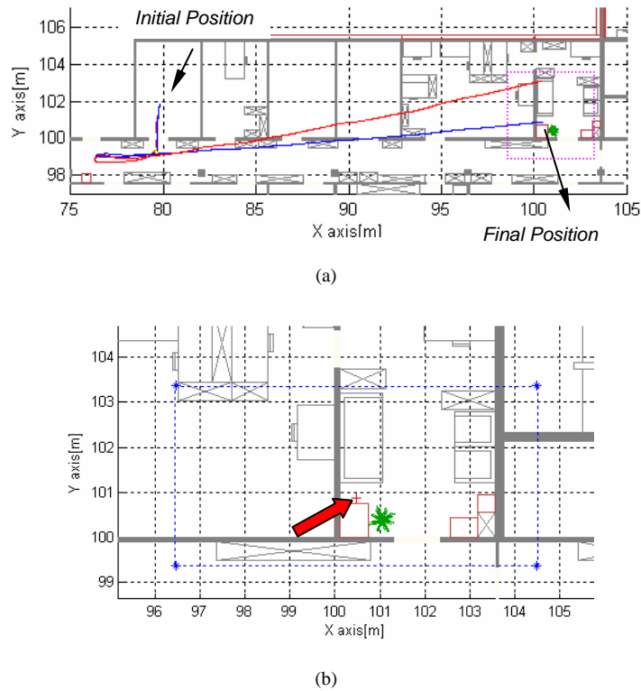
Figure 6. Trajectory generated by localization with odometry data, red line, in comparison with the trajectory resulted from laser data, blue line (a) and detail of laser data localization final position estimation (b).
