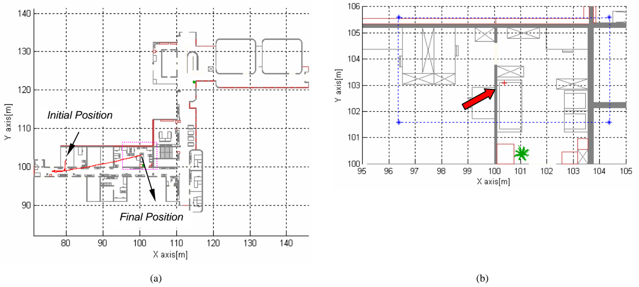
Figure 5. The mobile robot odometry-based resulted path (a) and detail of its final position according to odometry-based localization estimation (b) – red cross.
