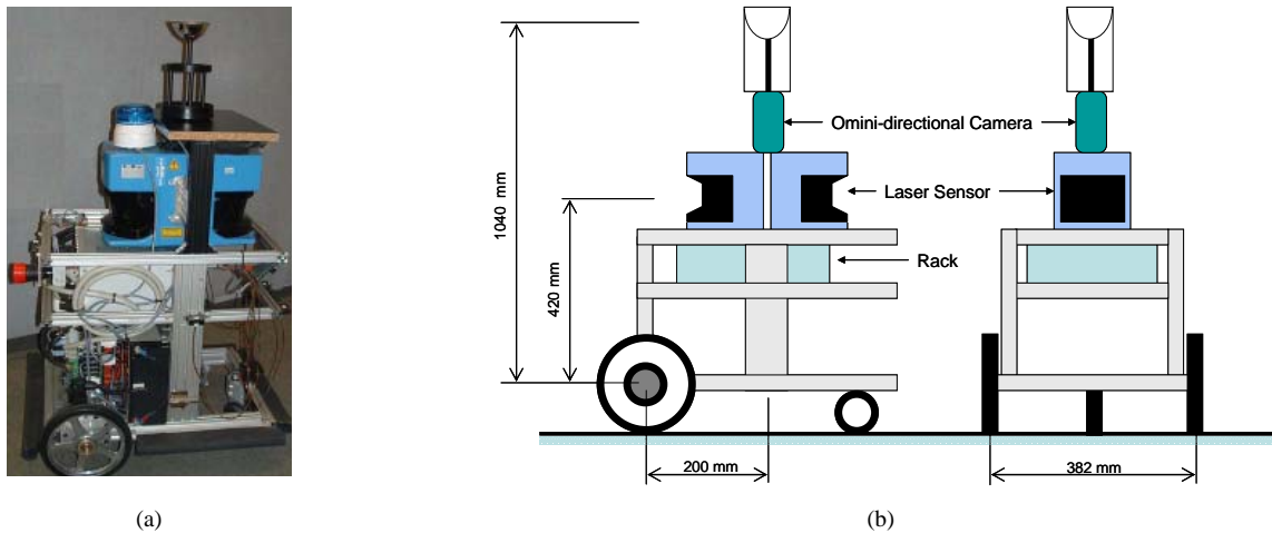
Figure 3. The BIBA robot.
