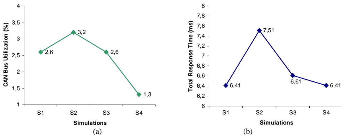
Figure 6 – Operational behavior of the CAN network with results of the simulation software (a) Graph of the bus utilization, (b) Graph of the total response time
