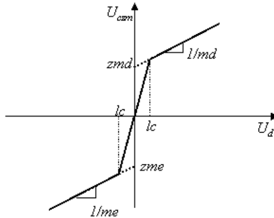
Figure (3). Graphical representation of the smoothed dead zone inverse.
