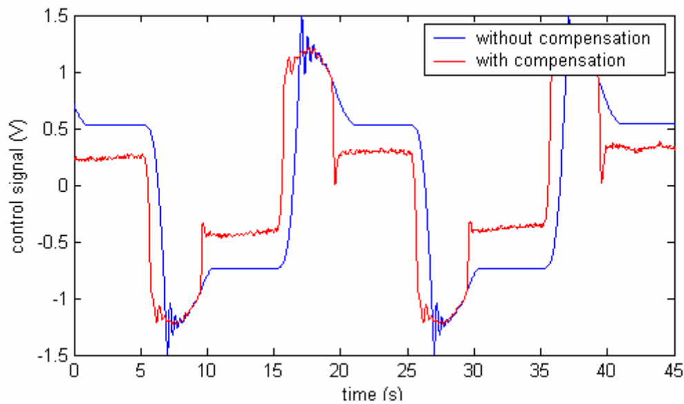
Figure 9. Control signal to polynomial trajectory
