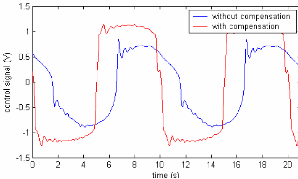
Figure 8. Control signal to sinusoidal trajectory
