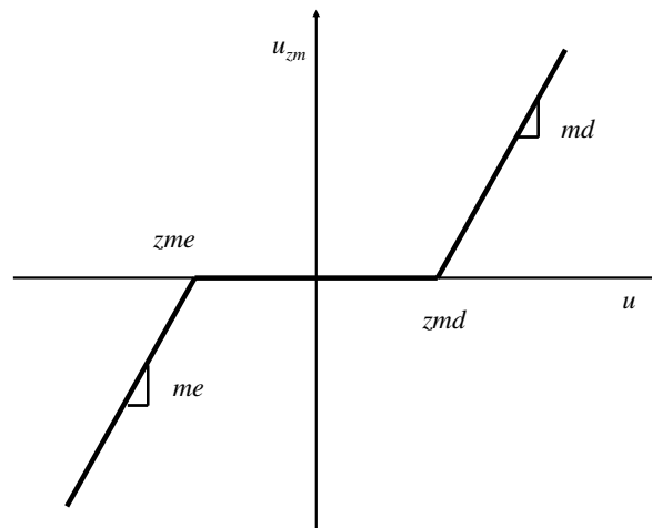
Figure 2. Graphical representation of the dead zone
