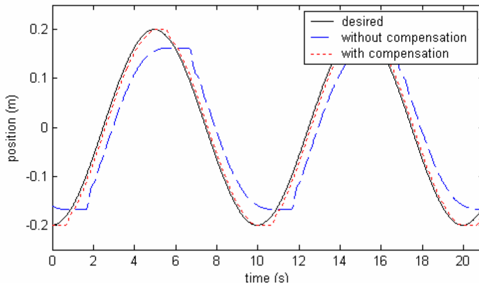
Figure 4. Experimental results to sinusoidal trajectory tracking
