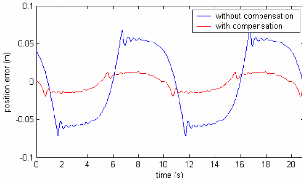
Figure 6. Position error to sinusoidal trajectory
