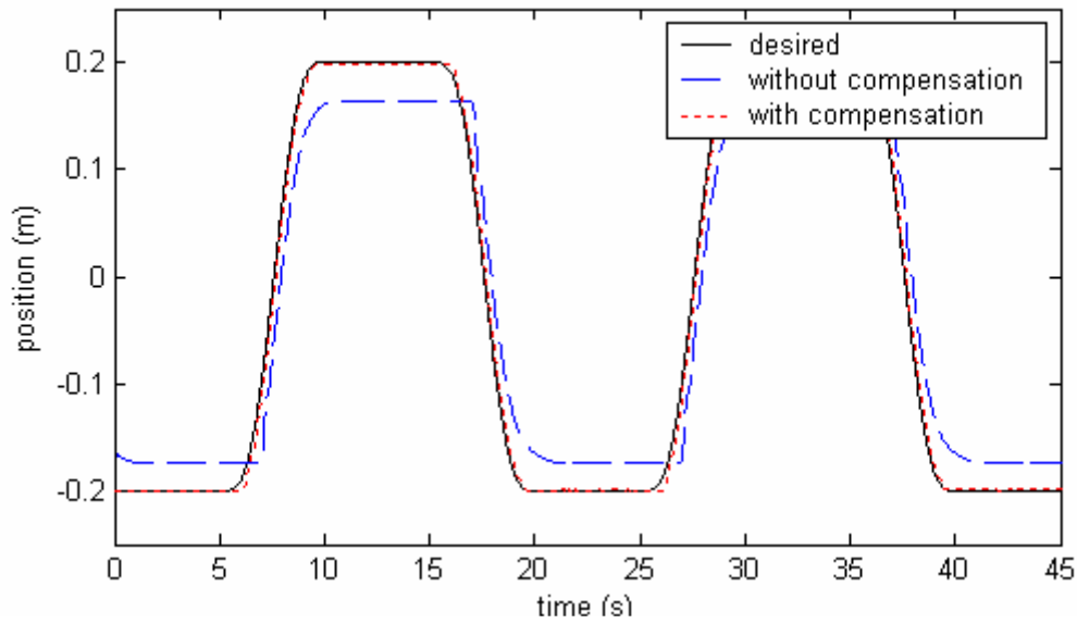
Figure 5. Experimental results to polynomial trajectory tracking
