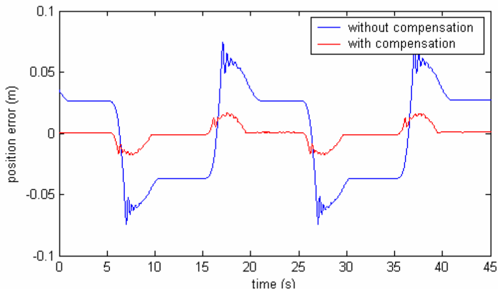
Figure 7. Position error to polynomial trajectory
