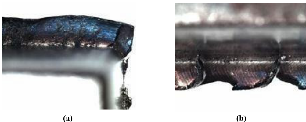
Figure 13. (a) Bottom view of the burr formed during test 16 at region 1 (Mag. 20X); (b) Bottom view of the burr formed during test 16 at region 2 (Mag. 15X)
