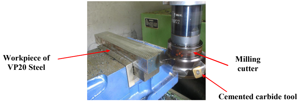
Figure 5. Set-up of the workpiece and the milling cutter
