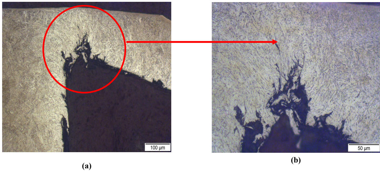
Figure 11. Detail of the burr root obtained at region1 of test 14: (a) magnification of 200X e (b) magnification of 500X
