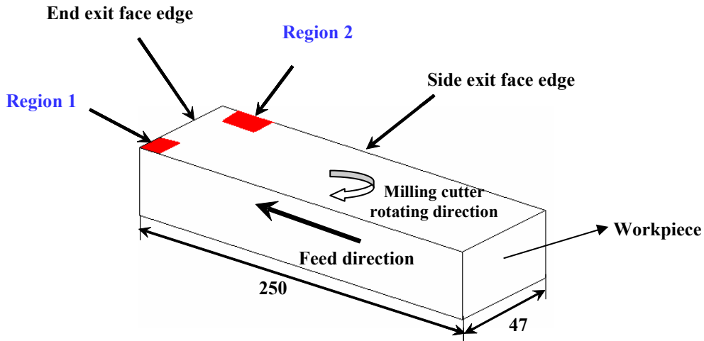
Figure 2. Identification of the regions where the burrs were reproduced for measuring their dimensions
