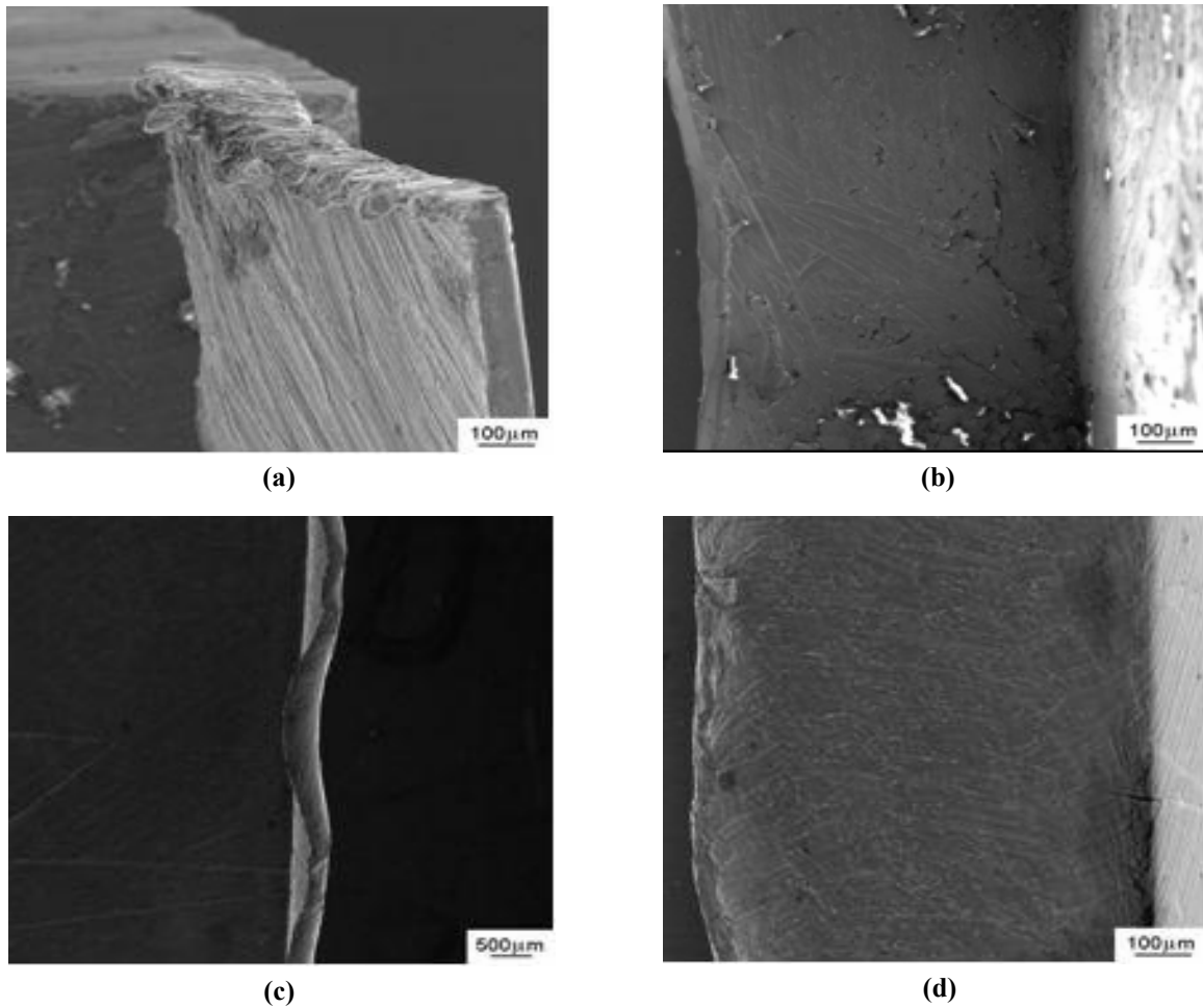
Figure 12. SEM photos of the burrs formed during test 14: (a) Burr at region 1 - rollover burr ; (b) Bottom view of the same burr; (c) Burr at region 2 - Wave-Type Burr ; (d) Bottom view of the same burr
