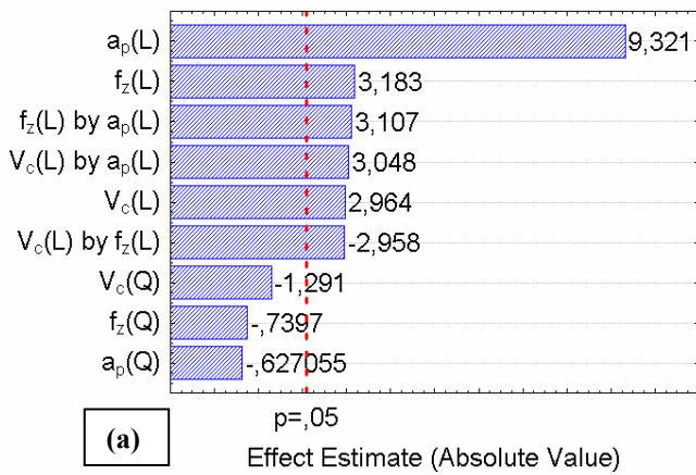
Pareto Chart of Standardized Effects; Variable: "h" (μm) 3 factors, 2 Blocks, 32 Runs; MS Residual=62380,9 DV: "h" (μm)
