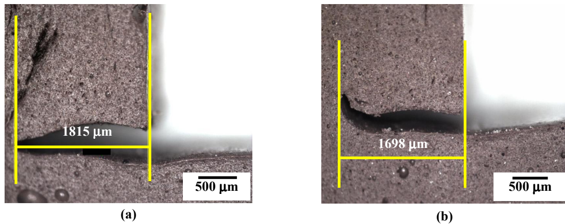
Figure 10. Dimensions of the burr generated during test 14 determined using the mold of polysulphide based mass (burr reproduction technique) (a) Region 1; (b) Region 2
