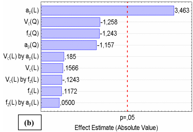
Pareto Chart of Standardized Effects; Variable: "h" (μm) 3 factors, 2 Blocks, 32 Runs; MS Residual=177046,9 DV: "h" (μm)
