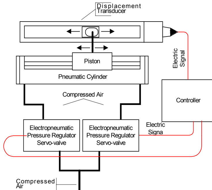
Figure 4. Pneumatic servo positioning system.
