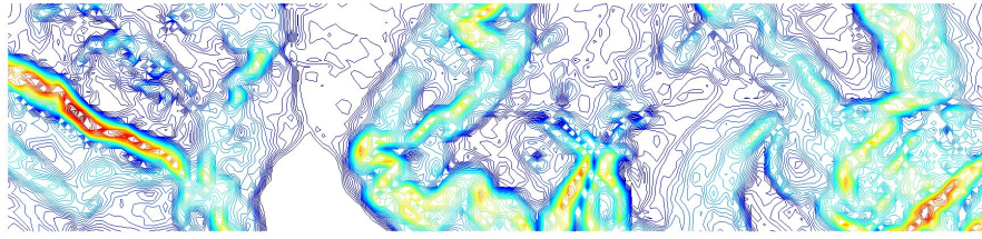
Figure 4. Isopotentials of orientation-invariant components of U_{rep\ total} computed for the terrain shown in Fig. 3.
